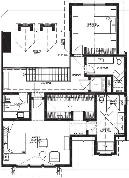
SECOND FLOOR ALTERNATIVE LAYOUT
