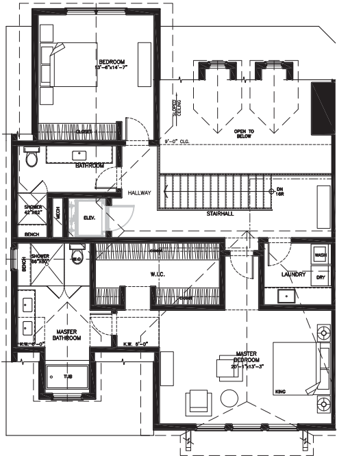
SECOND FLOOR ALTERNATIVE LAYOUT
