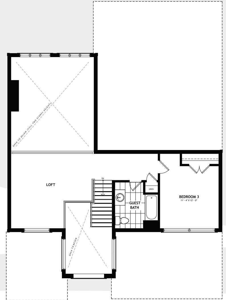
Second Floor Elevation B
