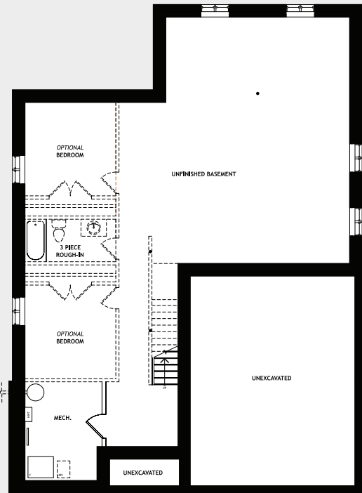
Basement Elevation B
