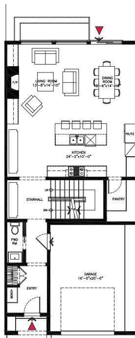
MAIN FLOOR
